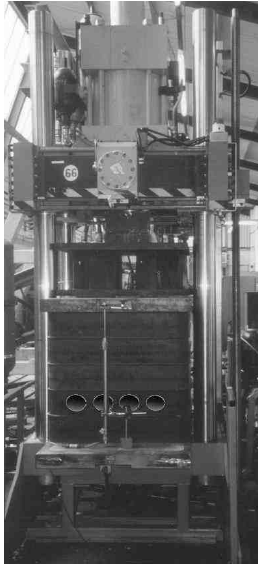
STAKKAbox ULTIMA CHAMBER 1500mm x 750mm UNDER VERTICAL LOADING
